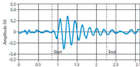
RF Waveform: #2 FBH @ 0.5"
