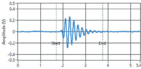
RF Waveform: Backwall signal from 1" steel block
