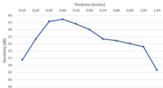
DAC Curve
